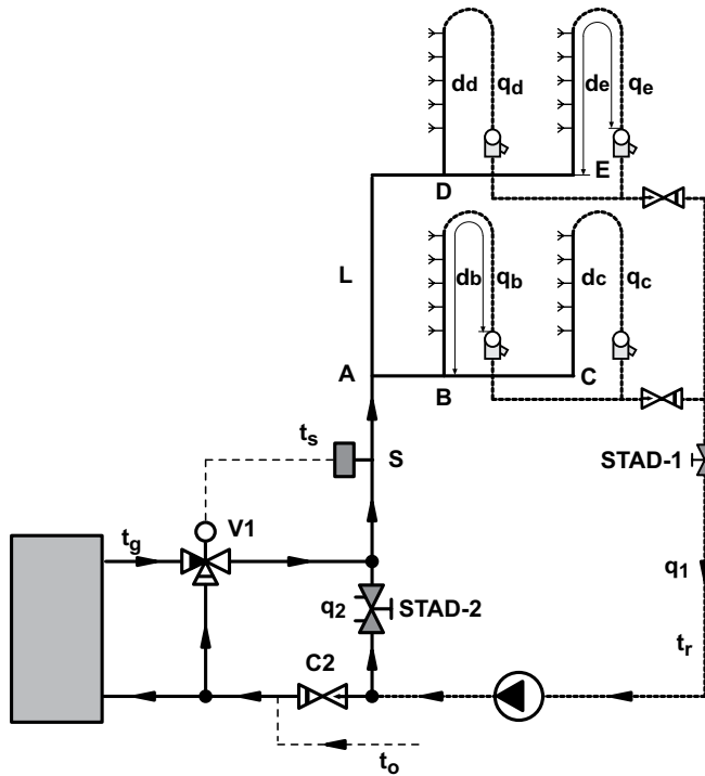
Fig 6.9: The return temperature of each branch is maintained automatically.
