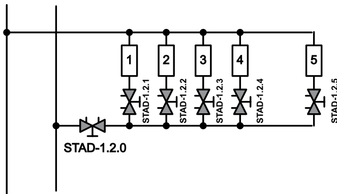
Fig 3.1: Balancing of terminals on a branch.
