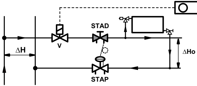
Fig 6.4c: The control valve is situated upstream the measuring valve STAD.
