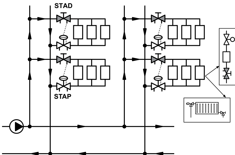
Fig 6.4a: A controller STAP stabilises the differential pressure on each branch.
