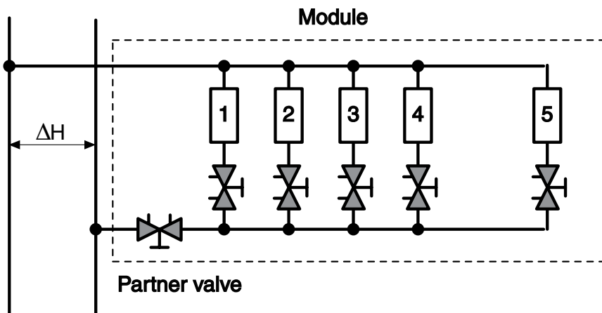
Fig 5.1: A module is created of several circuits connected to the same supply and return pipes.
