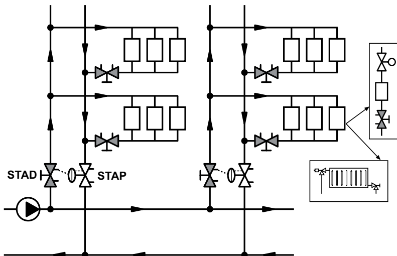
Fig 6.3: A controller STAP stabilises the differential pressure on each riser.
