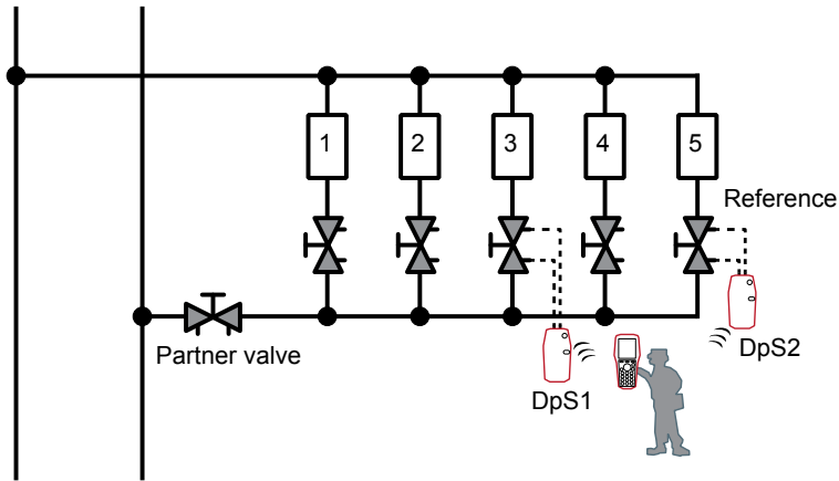
Fig 4.2: Balancing of terminals on a branch.
