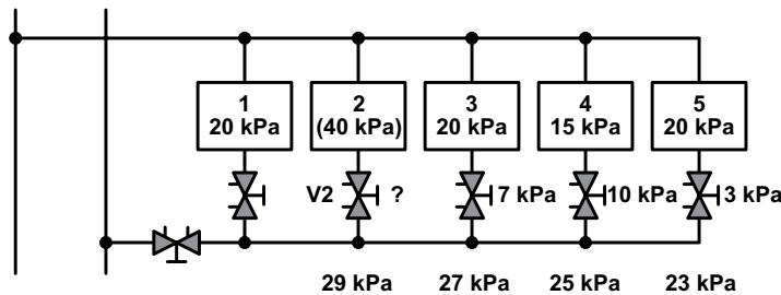
Fig 4.6: If 3 kPa is selected for the Reference valve, the differential pressure may be too low for the index circuit, here terminal 2.
