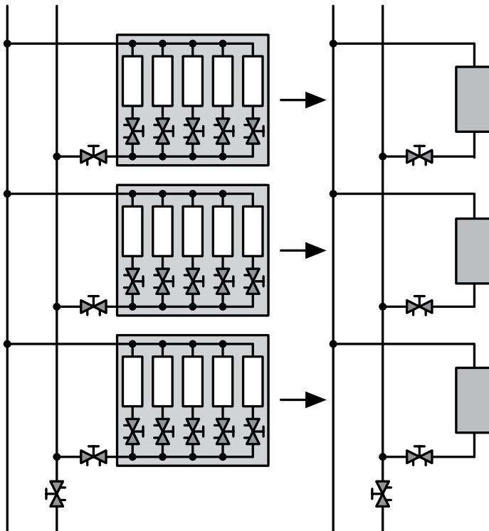
Fig 2.4: Each branch on a riser forms a new module.
