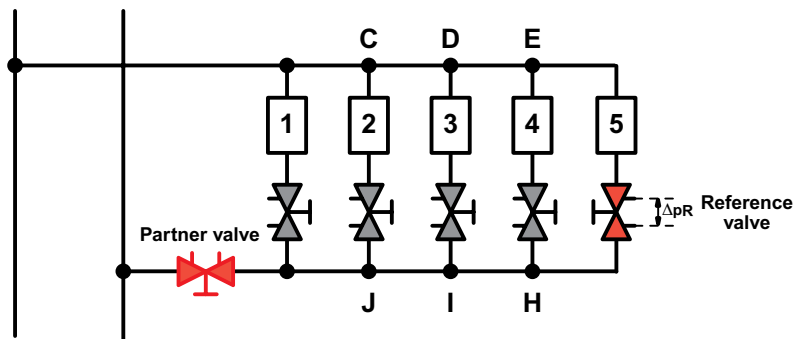
Fig 4.1: The Reference valve is always located in the module and on the terminal furthest away from the pump. The Partner valve determines the total flow in the branch.
