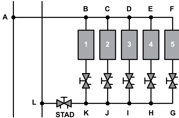
Fig 2.2: A branch with several terminals forms a balancing module. STAD is the Partner valve, which can compensate for external disturbances on the circuits already balanced.
