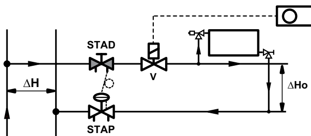
Fig 6.4b: Wrong design with the control valve situated downstream the measuring valve STAD.
