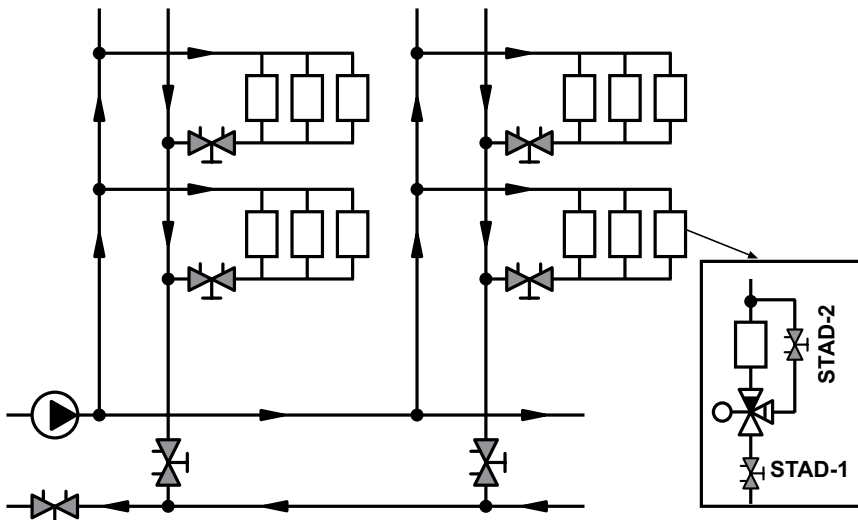
Fig 6.7: The primary flow is maintained constant with a three-way valve in diverting function on each terminal.
