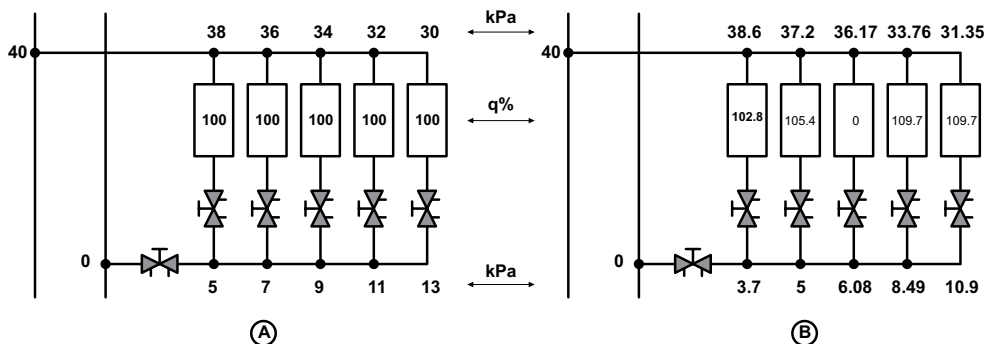
Fig 2.3: At an internal disturbance, the flows do not change in proportion to each other.
