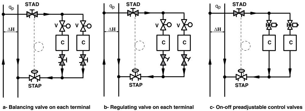
Fig F8: The STAD keeps the differential pressure constant across a set of terminal units.
