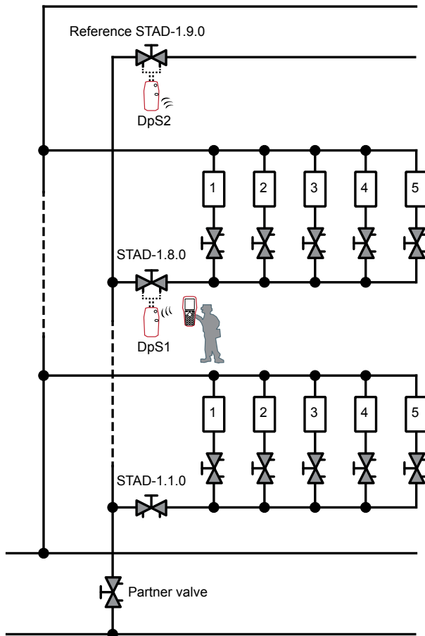
Fig 4.3: Balancing branches on a riser.
