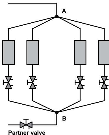
Fig 2.1: An external disturbance has the same effect on each terminal in the module.
