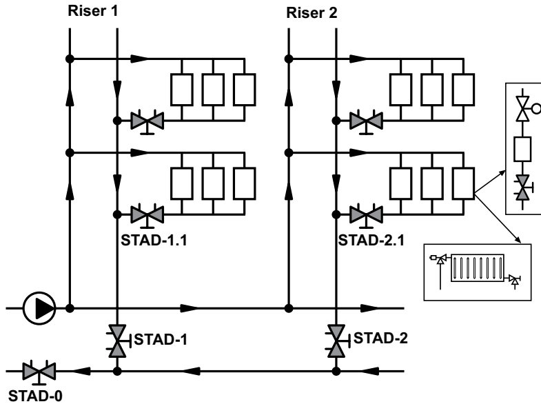
Fig 6.1: General example of a hydronic distribution.
