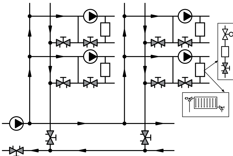
Fig 6.6: Constant flow distribution in the primary side and variable flow in the secondary circuits.
