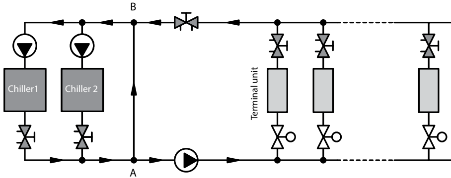
Fig F.2: Example of a variable flow distribution system.
