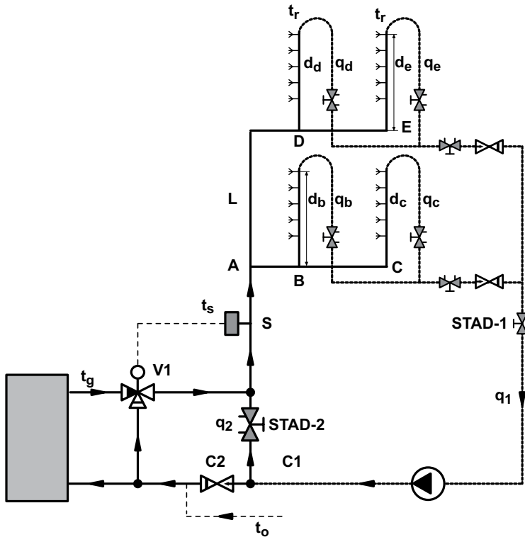
Fig 6.8a: A circulation pump maintains the temperature of water distribution.
