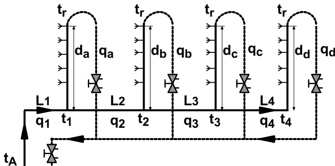
Fig 6.8b: One branch of the distribution with 4 circuits.
