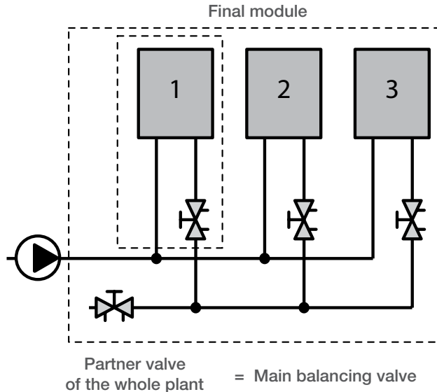
Fig 5.3: All the risers constitute the final module
