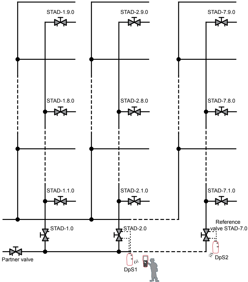
Fig 4.4: Balancing of risers.
