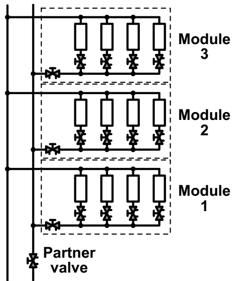
Fig 5.2: The riser module is created of modules 1, 2 and 3 when these are calculated and set.
