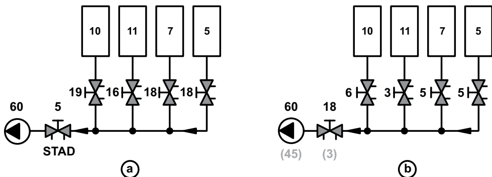
Fig 2.5: A set of terminals can be balanced in many ways, but only one is the optimum.
