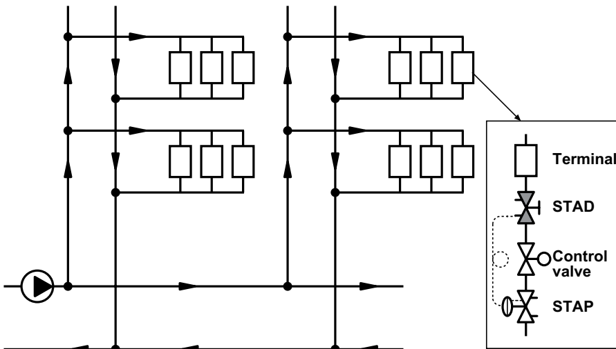
Fig 6.5: The differential pressure is kept constant on each control valve with a STAP.
