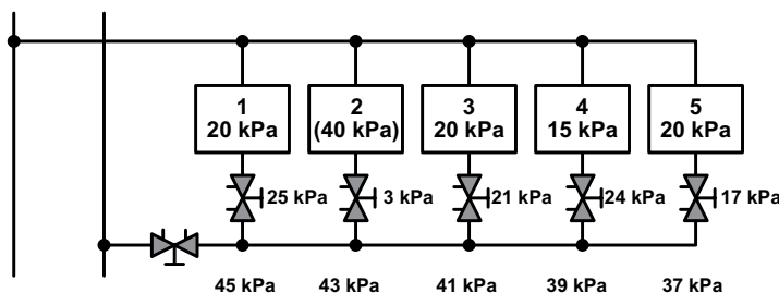
Fig 4.7: Differential pressure across circuits and pressure losses in balancing valves and terminals.
