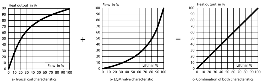
Fig F4: Adopting an inverse non-linear characteristic for the control valve compensates non-linearity of a coil characteristic.
